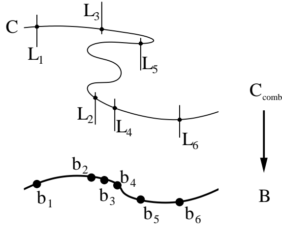
FIGURE 3. A comb is a linked curve where every link, or tooth, intersects the handle precisely once.
