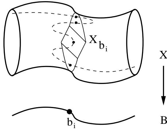
FIGURE 5. Where a log preflexible curve intersects a nonreduced fiber—e.g., the middle component has multiplicity 2—the map from the curve to B is necessarily ramified.
