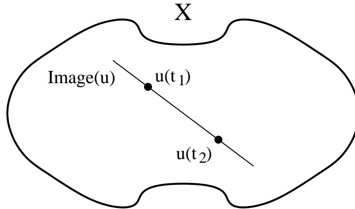
FIGURE 1. Every pair of points in a rationally connected variety lies in an image of the projective line.
