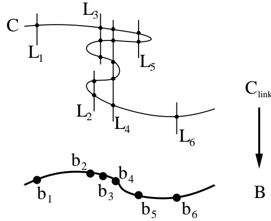
FIGURE 2. A linked curve with handle C and some links intersecting C in more than 1 point.
