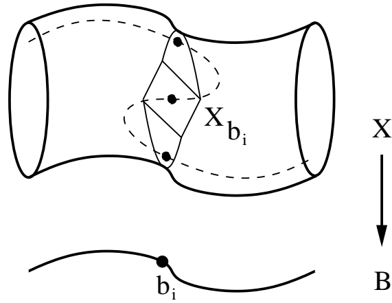
FIGURE 4. Where a log preflexible curve intersects a reduced, possibly singular, fiber the map from the curve to B is unramified.
